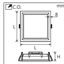
square recessed (SQ.RCS)
